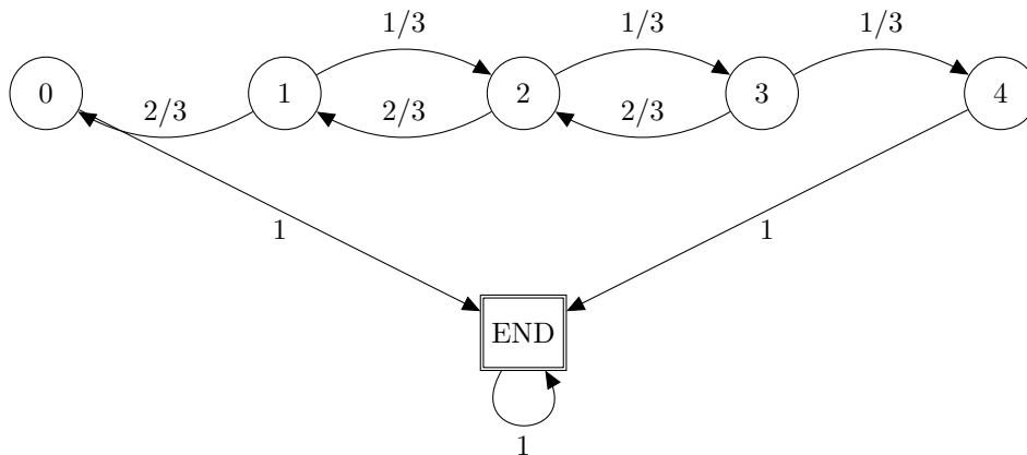
Figure 1: Gambler's Ruin: N = 4 . An absorbing state s \in S is s.t. P[s | s] = 1 . The END state is an absorbing state in Gambler's Ruin.
